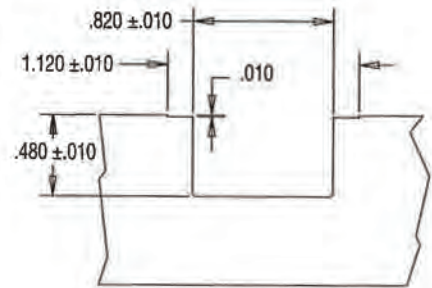
Panel Cutout .057 ± .002 Thickness
