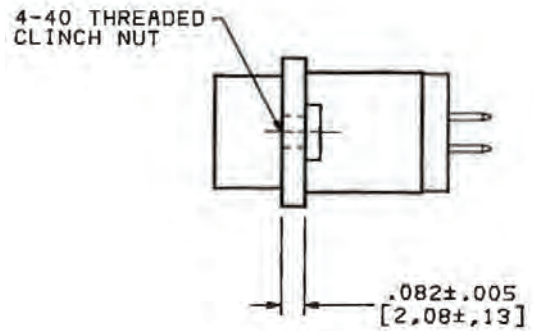
Mounting Style 2
