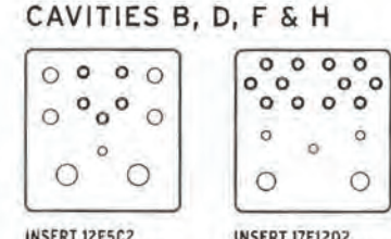
INSERT 12F5C2 (5) SIZE 16 FIBRE OPTIC (1) SIZE 16 (4) SIZE 12 (2) SIZE 5 COAX
